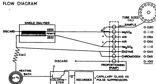
FLOW DIAGRAM
