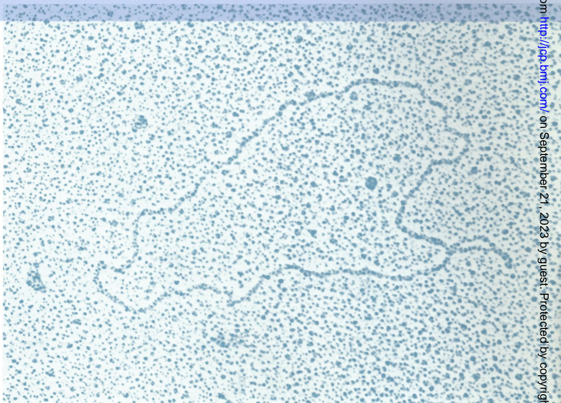
Electromicrograph of plasmid DNA from a strain of Staphylococcus aureus in covalently open circular form. See fig (b), page 902
