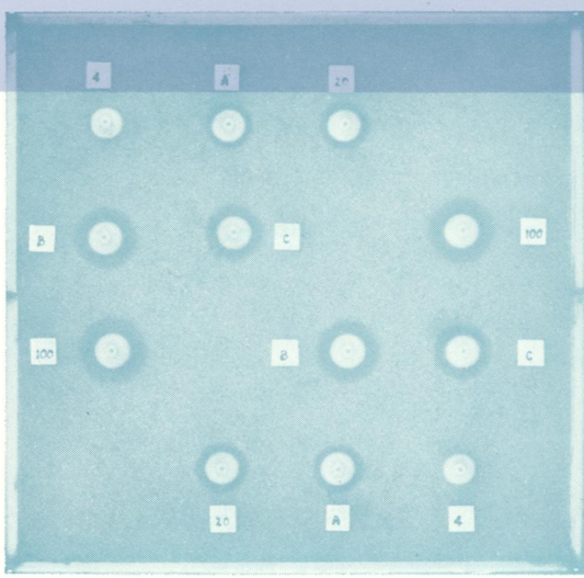
(Left) 5-fluorocytosine assay Standards: 4, 20, 100 \mu\text{g/ml} 5-FC in serum Test sera: A, B, C Diagonal replication: C. pseudotropicalis (Right) Clotrimazole assay Standards: 0.01, 0.05, 0.2, 1.0 \mu\text{g/ml} in serum Test sera: A, B C. pseudotropicalis. See figs 3 and 4, page 772.
